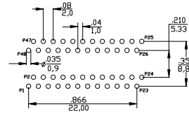
recommend PCB layout
